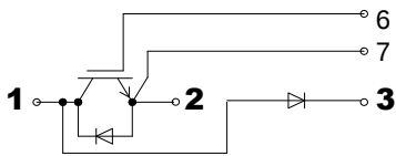
SGD145T60UC1 (Boost Chopper)
