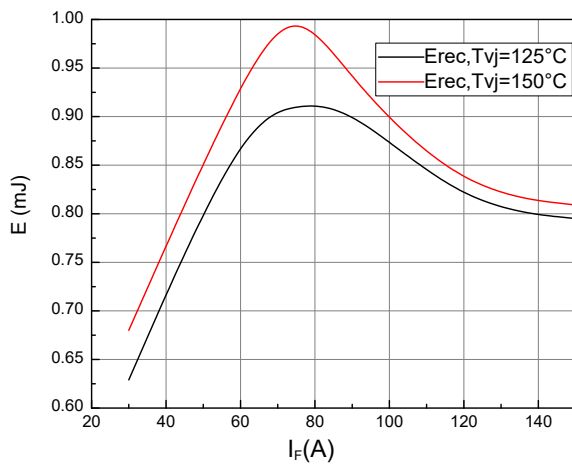
Fig. 7. Switching losses of Diode R_{g, on}=8\Omega, V_{CE}=400\text{V}
